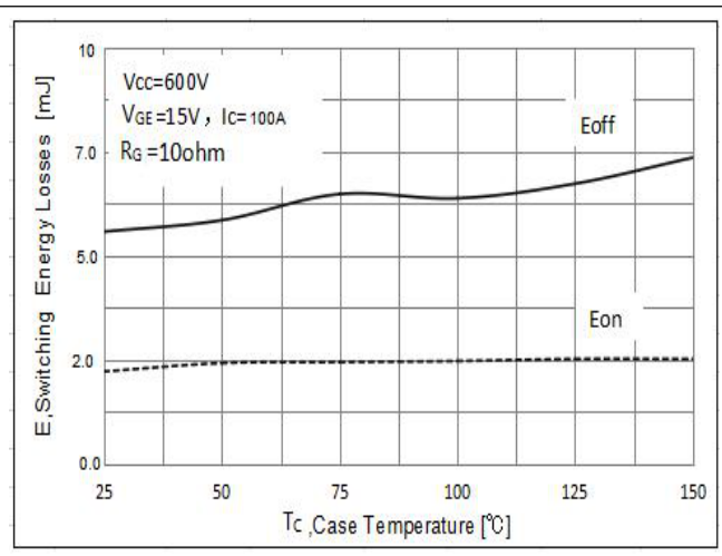
Typical switching energy losses as a function of Case Temperature
