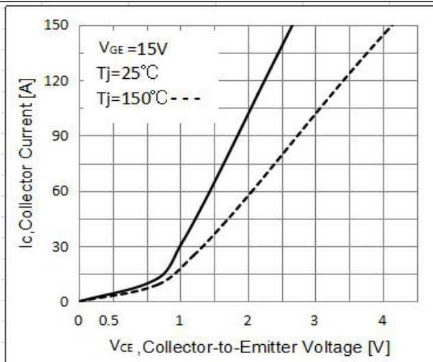
Collector-emitter saturation voltage Characteristic
