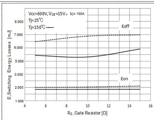
Typical switching energy losses as a function of gate resistor
