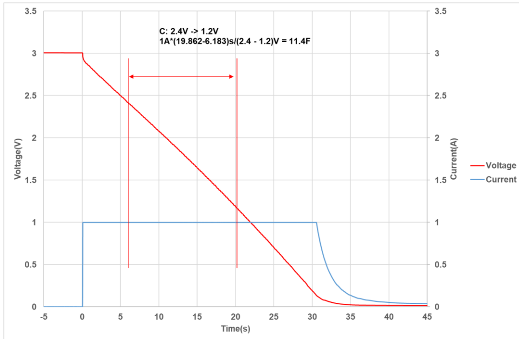
Fig 1: Capacitance measurement
