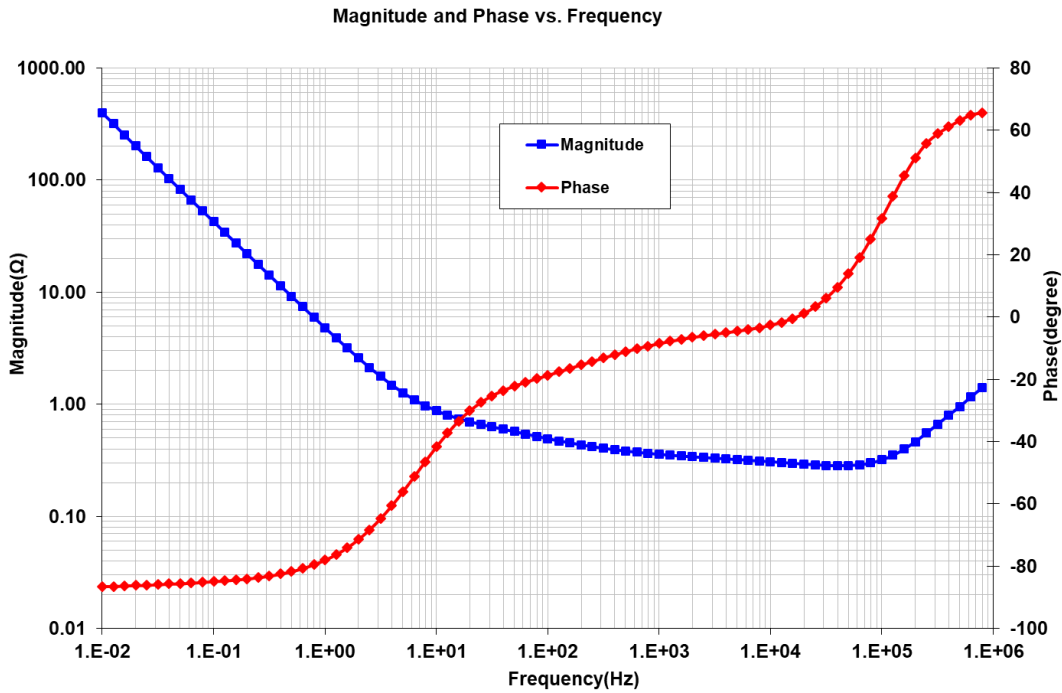
Fig 8: Frequency Response of Impedance (biased at 4.5V with a 50mV test signal)
